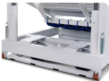
Dynamic Sub Frame in mobile position (up). Increased clearance space between DSF bar and floor allows for easy transport. Double swivel wheels help protect floors. Two rollers protect the DSF when driving up a ramp.
